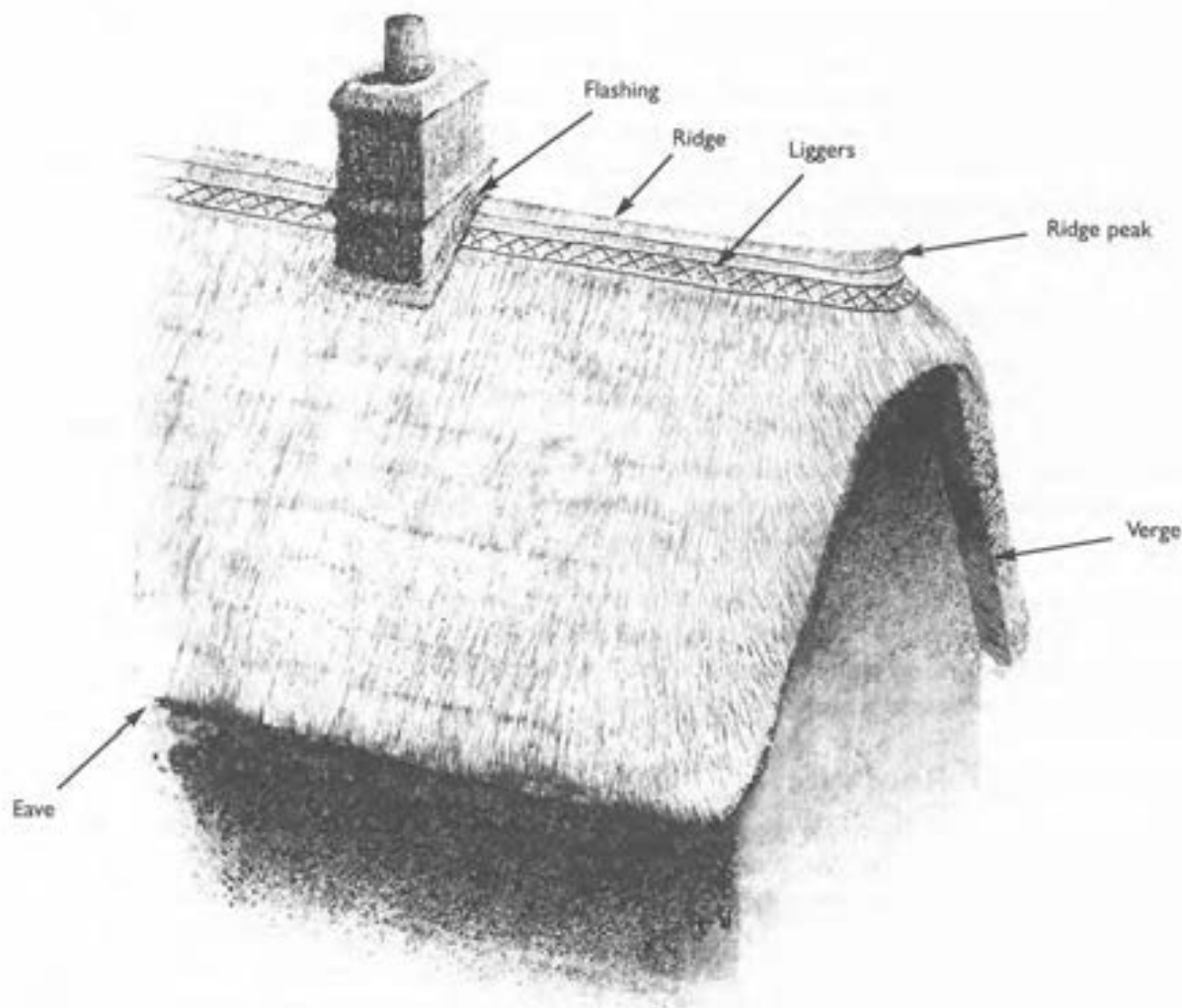
Drawing 1 - External features of a thatched roof
